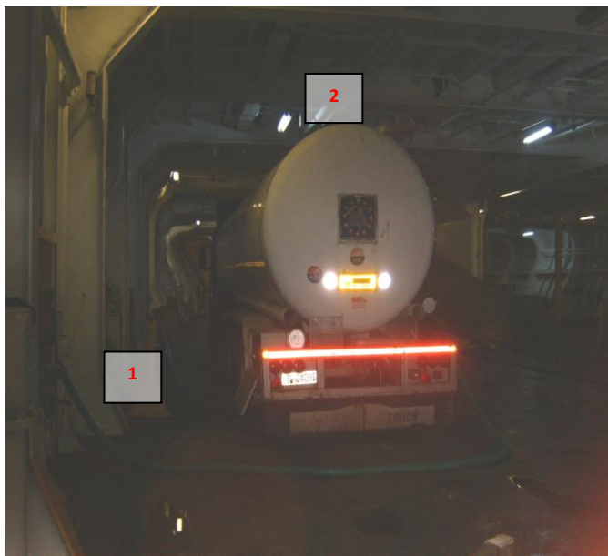
Picture 1: The tank truck parked near the water inlet valve, inside the garage of the Ro-Pax “NISSOS RODOS”. The water pipe, connected to the ship’s fresh water inlet valve is noticed. The position of the Boatswain (1) and the position of the driver (2) during the development of the accident have been marked.
